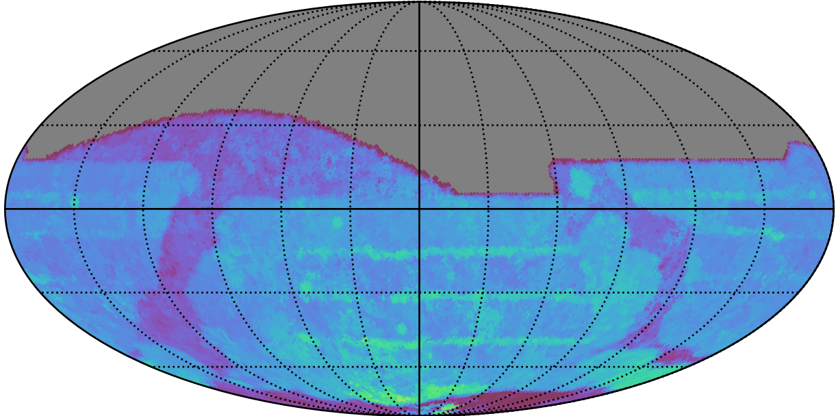
too_elab_r128_d2_griz_v3.4_10yrs All sky r band: 80thPercentile Season Length
