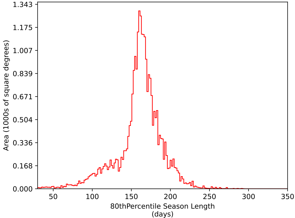
too_elab_r128_d2_griz_v3.4_10yrs All sky i band: 80thPercentile Season Length
