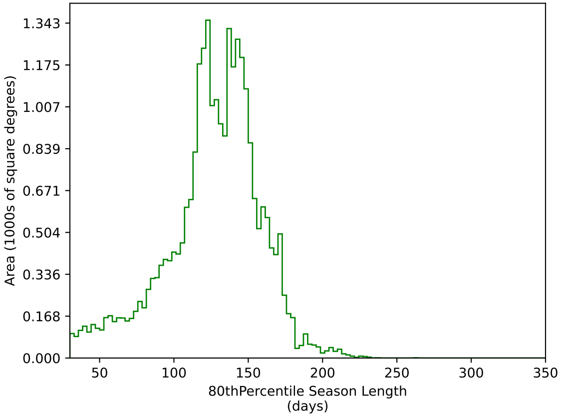
too_elab_r128_d2_griz_v3.4_10yrs All sky g band: 80thPercentile Season Length
