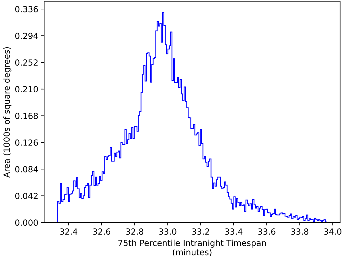
too_elab_r128_d2_griz_v3.4_10yrs WFD y band: 75th Percentile Intranight Timespan
