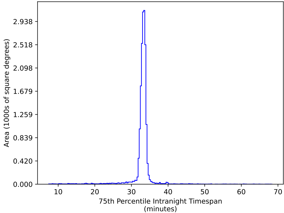
too_elab_r128_d2_griz_v3.4_10yrs WFD ug bands: 75th Percentile Intranight Timespan
