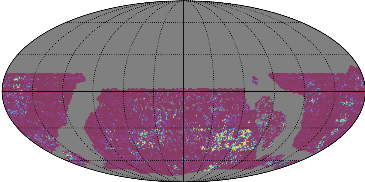
too_elab_r128_d2_griz_v3.4_10yrs WFD u band: 75th Percentile Intranight Timespan
