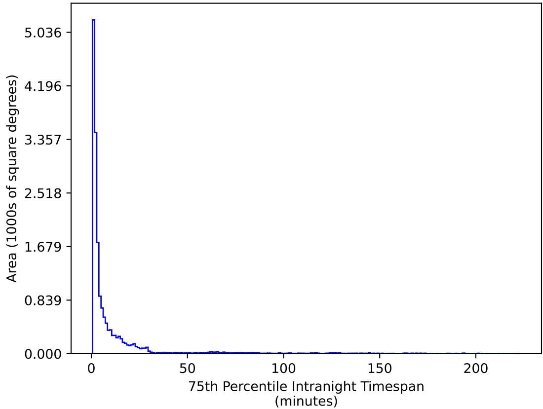
too_elab_r128_d2_griz_v3.4_10yrs WFD u band: 75th Percentile Intranight Timespan
