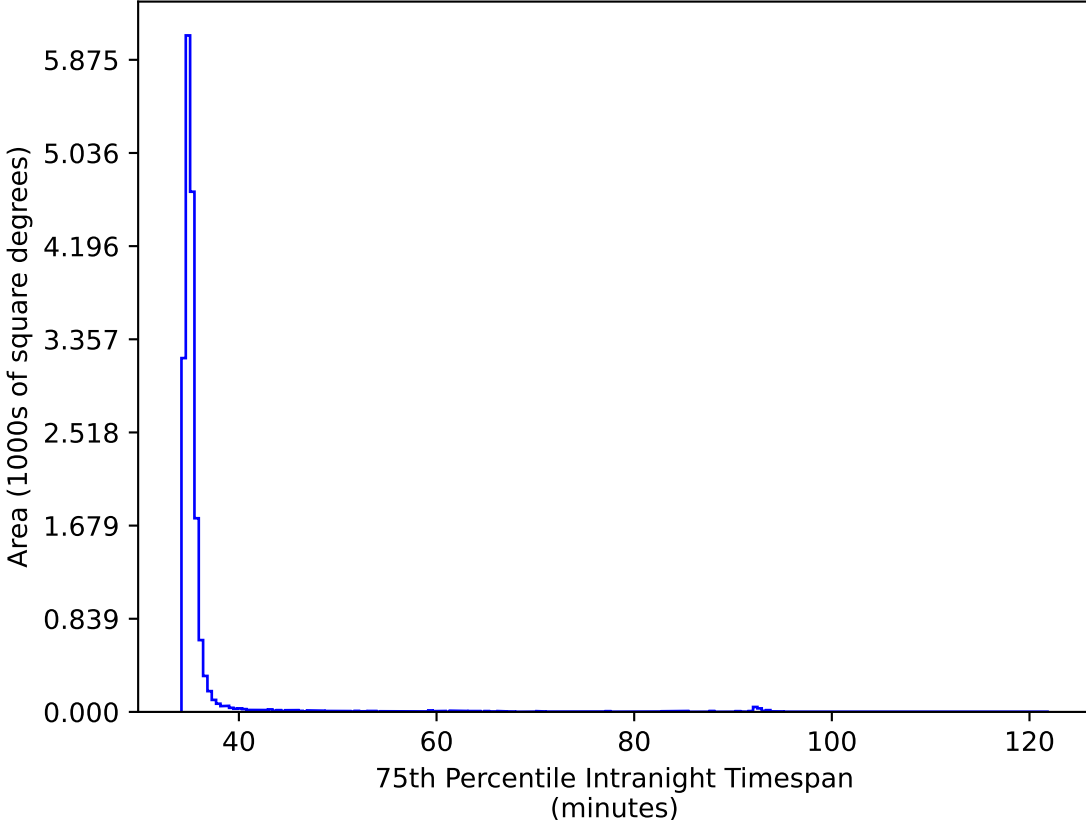
too_elab_r128_d2_griz_v3.4_10yrs WFD ri bands: 75th Percentile Intranight Timespan
