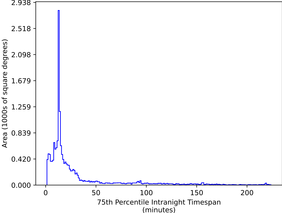
too_elab_r128_d2_griz_v3.4_10yrs WFD i band: 75th Percentile Intranight Timespan
