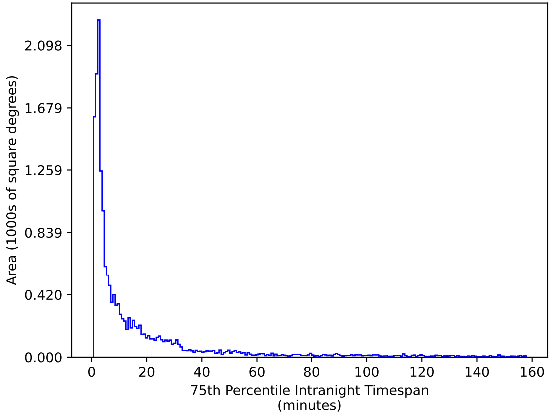
too_elab_r128_d2_griz_v3.4_10yrs WFD g band: 75th Percentile Intranight Timespan
