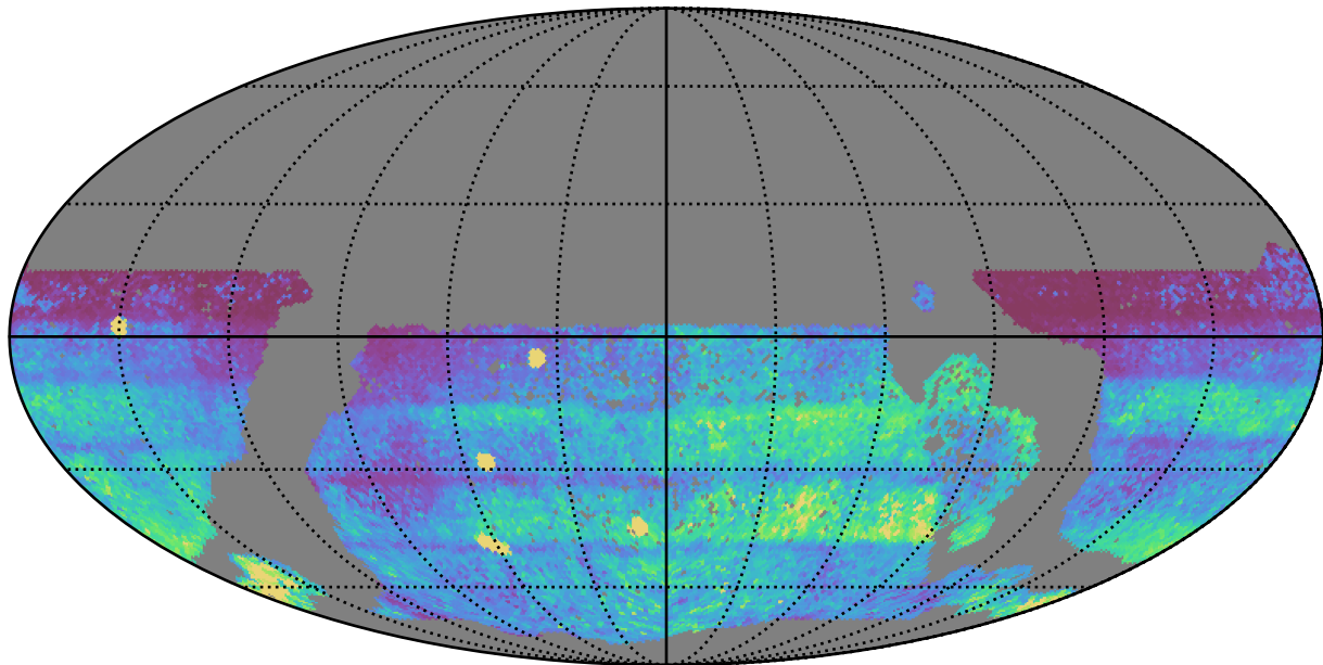
too_elab_r128_d2_griz_v3.4_10yrs WFD all bands: 75th Percentile Intranight Timespan
