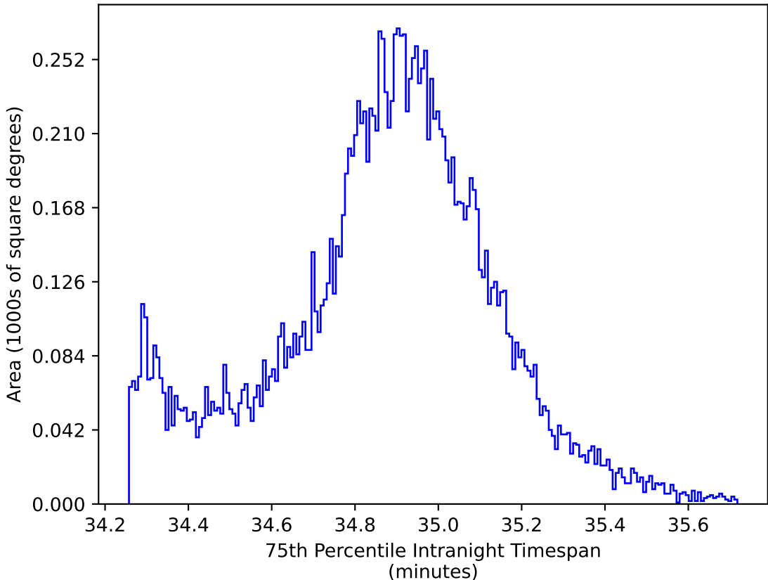
too_elab_r128_d2_griz_v3.4_10yrs WFD: 75th Percentile Intranight Timespan
