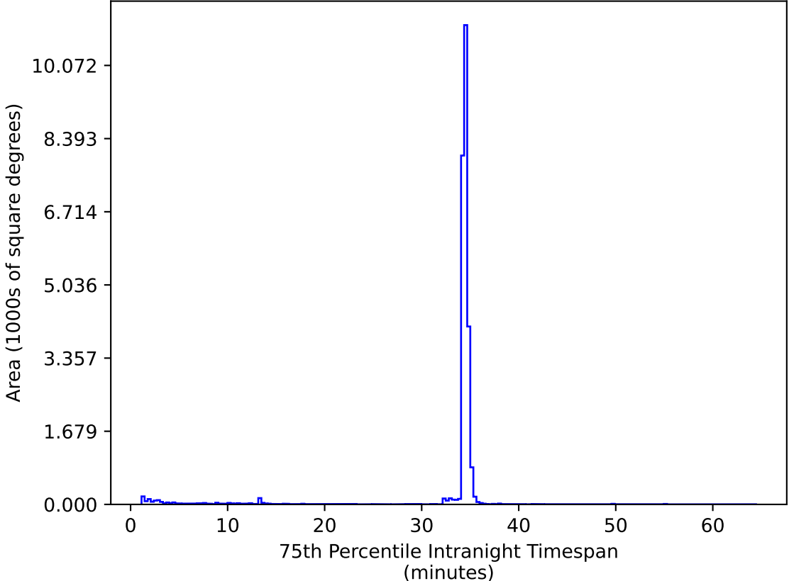
too_elab_r128_d2_griz_v3.4_10yrs All sky zy bands: 75th Percentile Intranight Timespan
