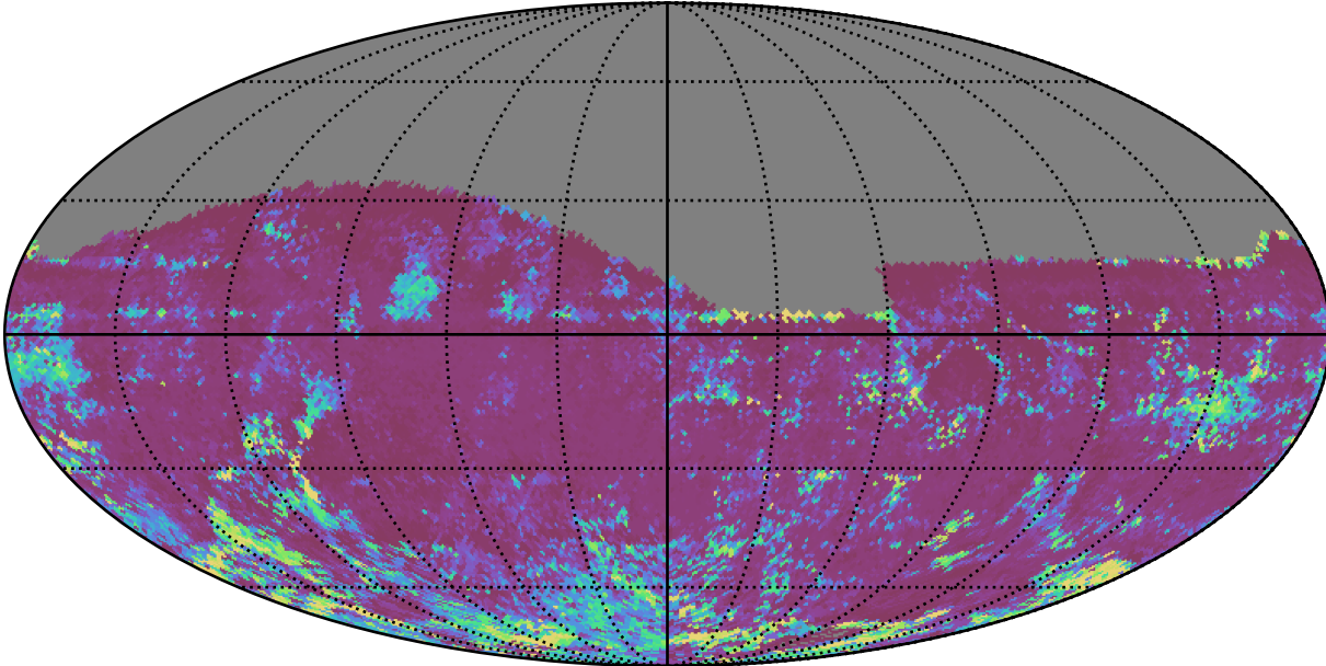
too_elab_r128_d2_griz_v3.4_10yrs All sky z band: 75th Percentile Intranight Timespan
