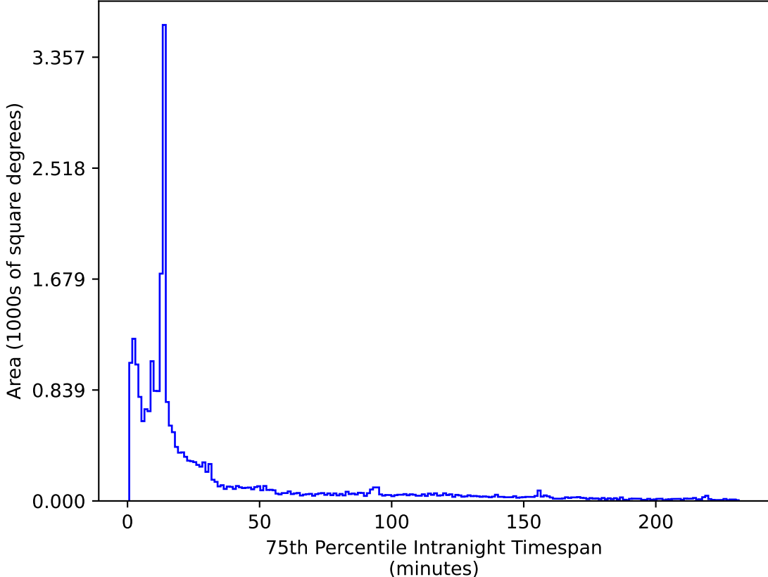
too_elab_r128_d2_griz_v3.4_10yrs All sky z band: 75th Percentile Intranight Timespan
