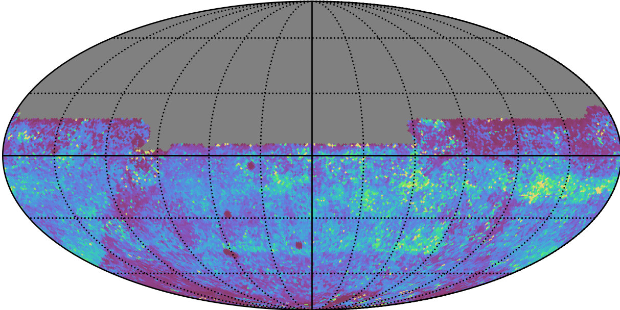
too_elab_r128_d2_griz_v3.4_10yrs All sky y band: 75th Percentile Intranight Timespan
