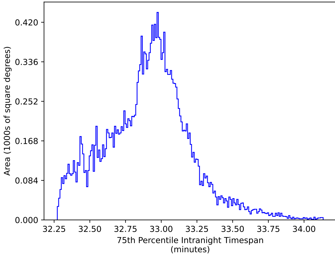
too_elab_r128_d2_griz_v3.4_10yrs All sky y band: 75th Percentile Intranight Timespan
