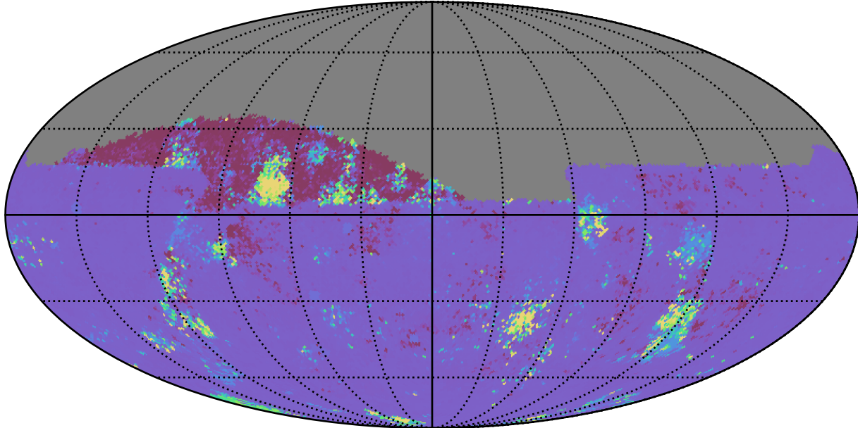
too_elab_r128_d2_griz_v3.4_10yrs All sky ug bands: 75th Percentile Intranight Timespan
