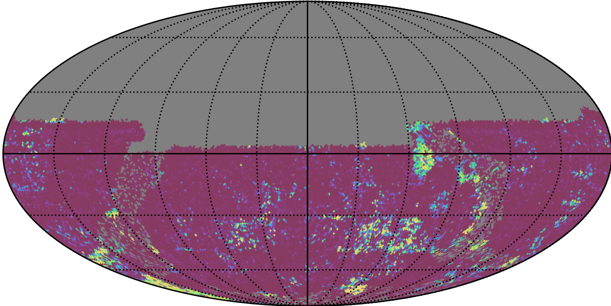
too_elab_r128_d2_griz_v3.4_10yrs All sky u band: 75th Percentile Intranight Timespan
