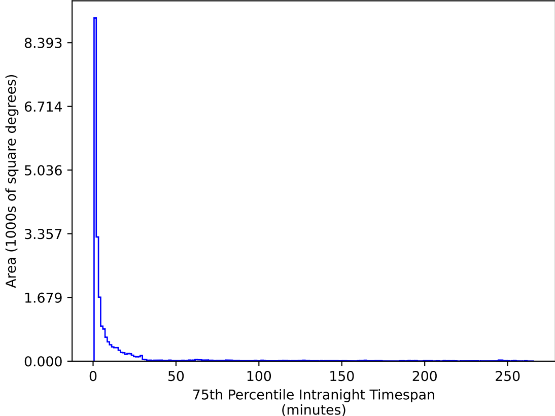
too_elab_r128_d2_griz_v3.4_10yrs All sky u band: 75th Percentile Intranight Timespan
