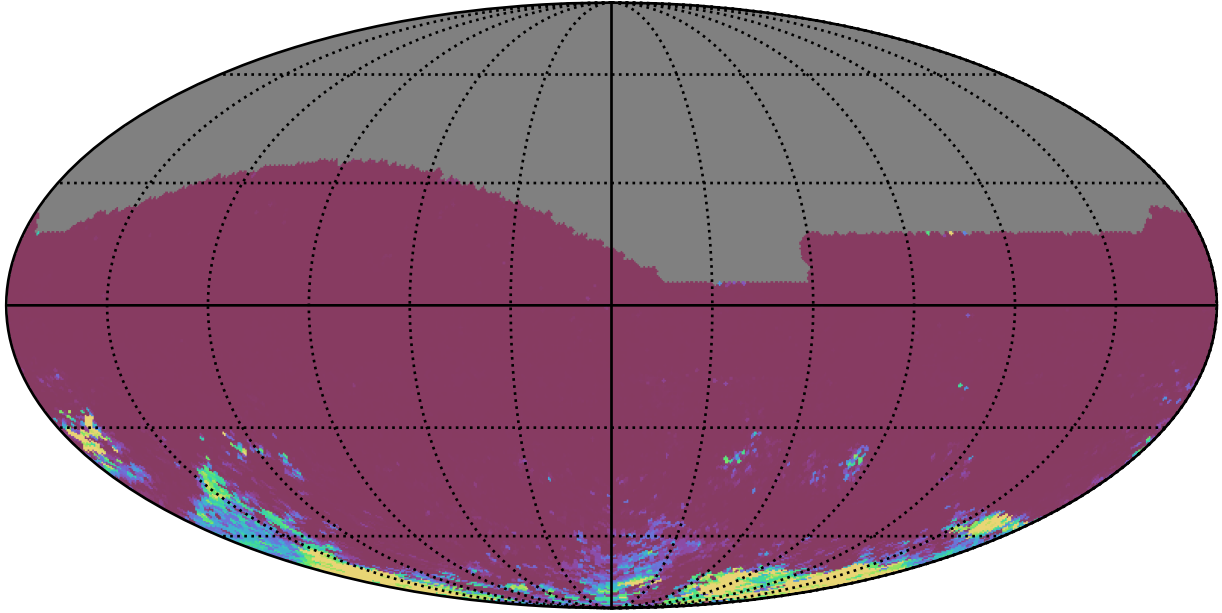
too_elab_r128_d2_griz_v3.4_10yrs All sky ri bands: 75th Percentile Intranight Timespan
