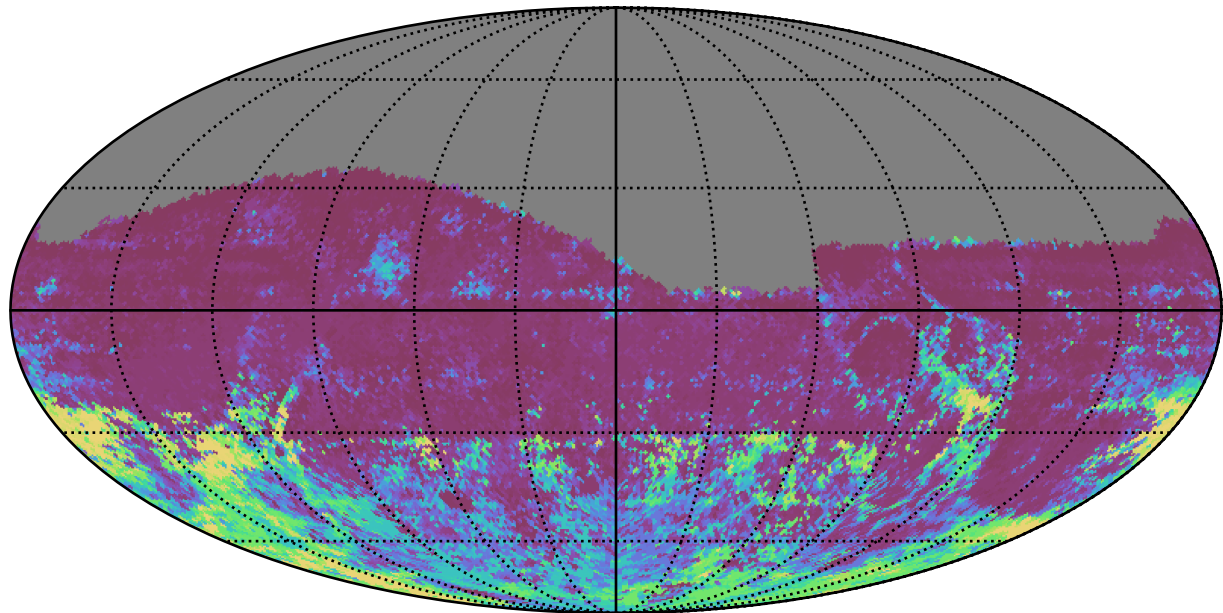
too_elab_r128_d2_griz_v3.4_10yrs All sky r band: 75th Percentile Intranight Timespan
