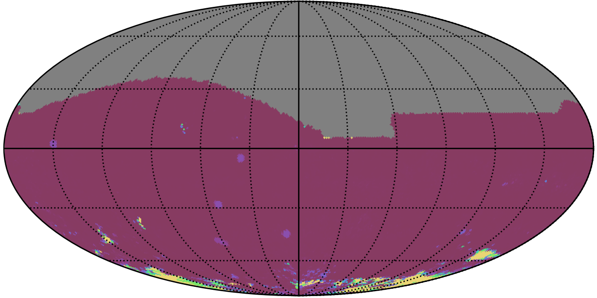
too_elab_r128_d2_griz_v3.4_10yrs All sky iz bands: 75th Percentile Intranight Timespan
