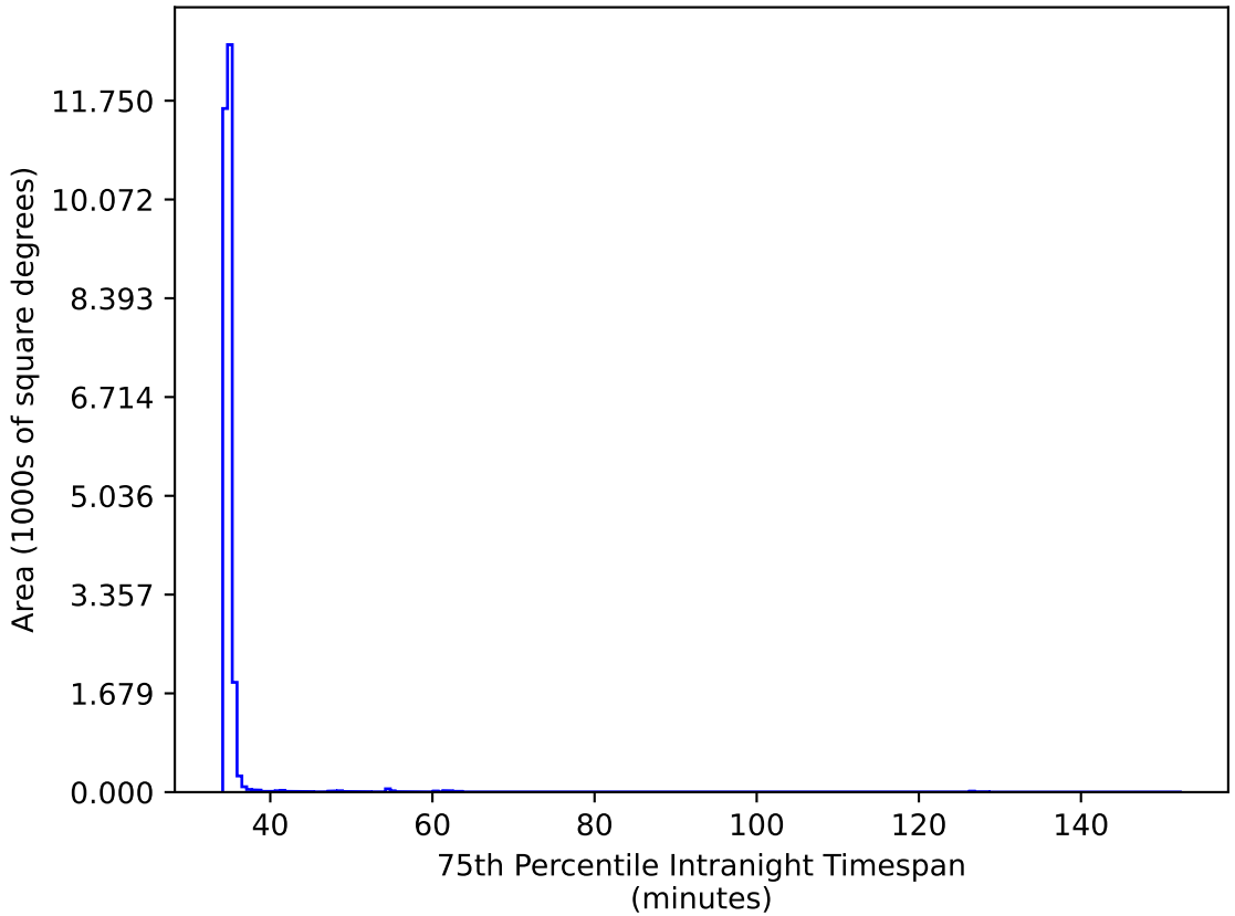
too_elab_r128_d2_griz_v3.4_10yrs All sky iz bands: 75th Percentile Intranight Timespan
