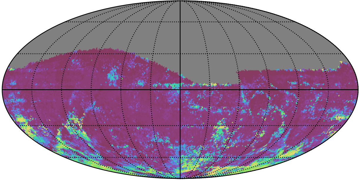
too_elab_r128_d2_griz_v3.4_10yrs All sky i band: 75th Percentile Intranight Timespan
