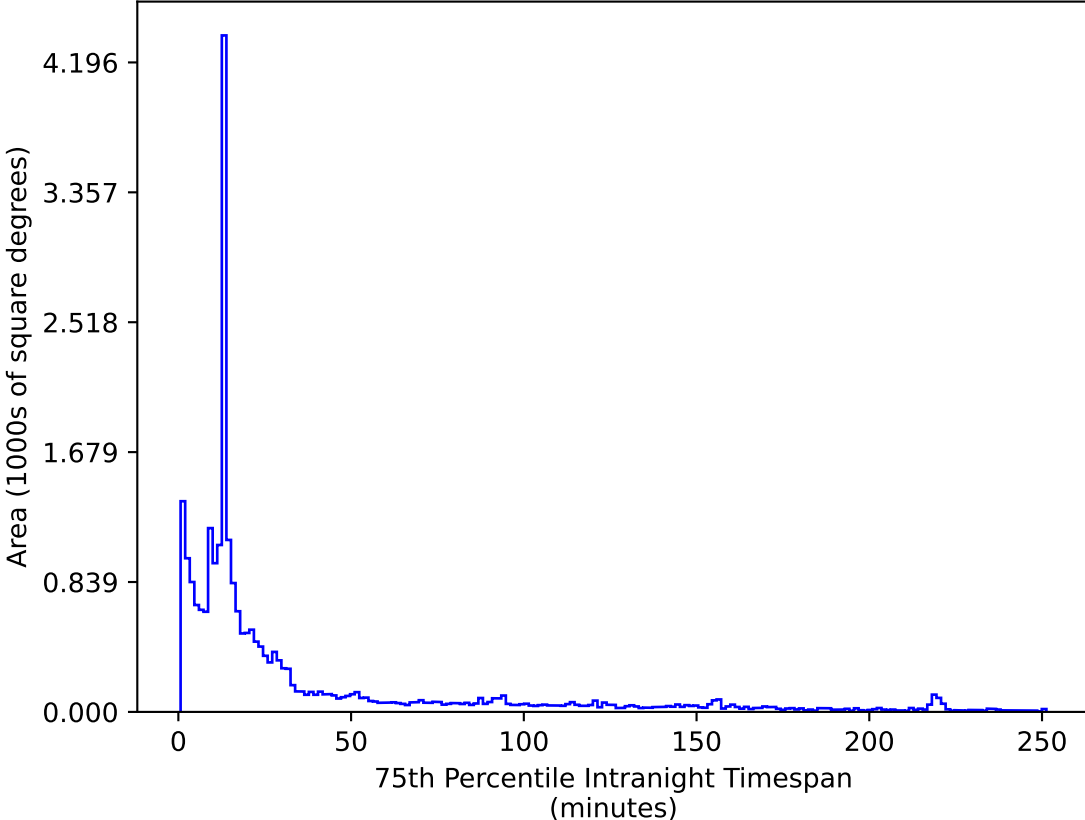
too_elab_r128_d2_griz_v3.4_10yrs All sky i band: 75th Percentile Intranight Timespan
