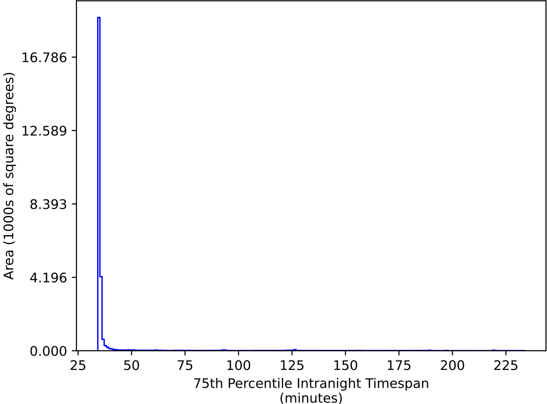
too_elab_r128_d2_griz_v3.4_10yrs All sky gr bands: 75th Percentile Intranight Timespan
