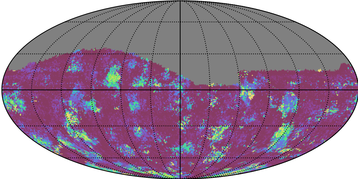
too_elab_r128_d2_griz_v3.4_10yrs All sky g band: 75th Percentile Intranight Timespan
