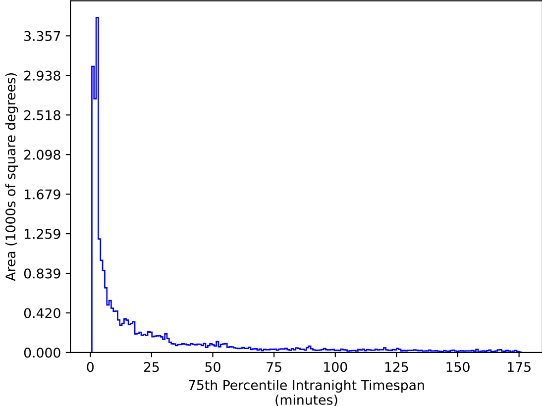
too_elab_r128_d2_griz_v3.4_10yrs All sky g band: 75th Percentile Intranight Timespan
