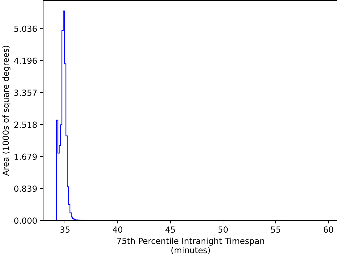
too_elab_r128_d2_griz_v3.4_10yrs All sky: 75th Percentile Intranight Timespan
