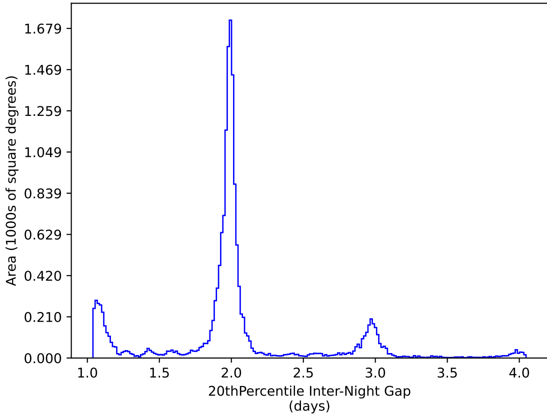
too_elab_r128_d2_griz_v3.4_10yrs WFD y band: 20thPercentile Inter-Night Gap
