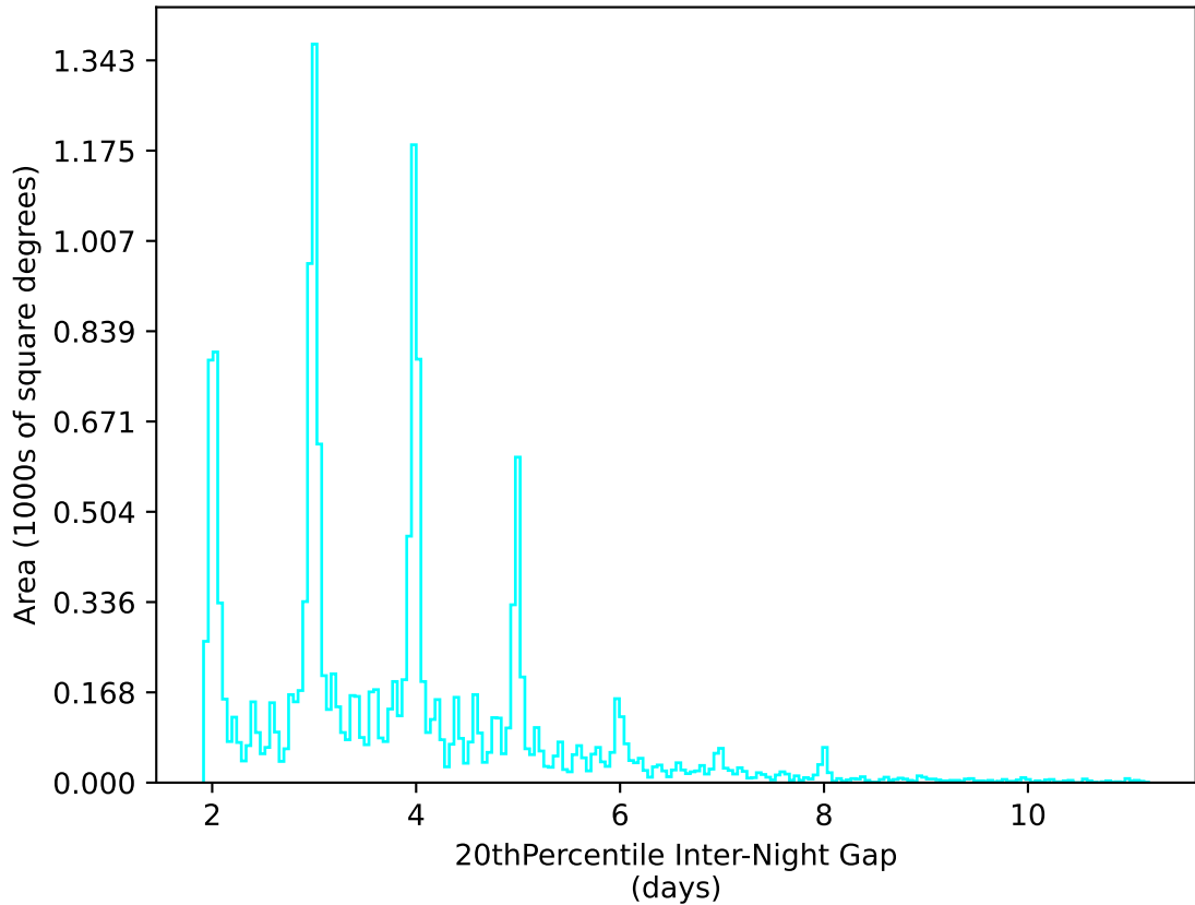
too_elab_r128_d2_griz_v3.4_10yrs WFD u band: 20thPercentile Inter-Night Gap
