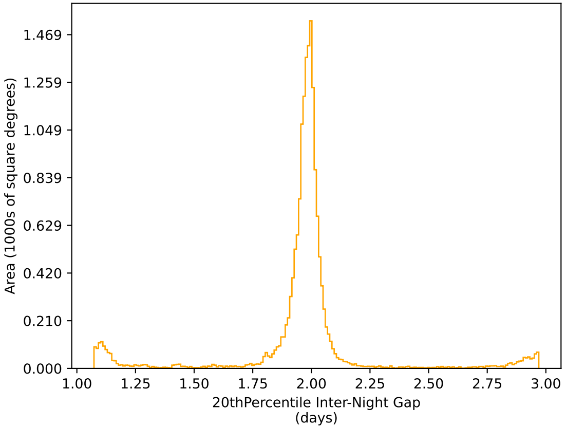
too_elab_r128_d2_griz_v3.4_10yrs WFD r band: 20thPercentile Inter-Night Gap
