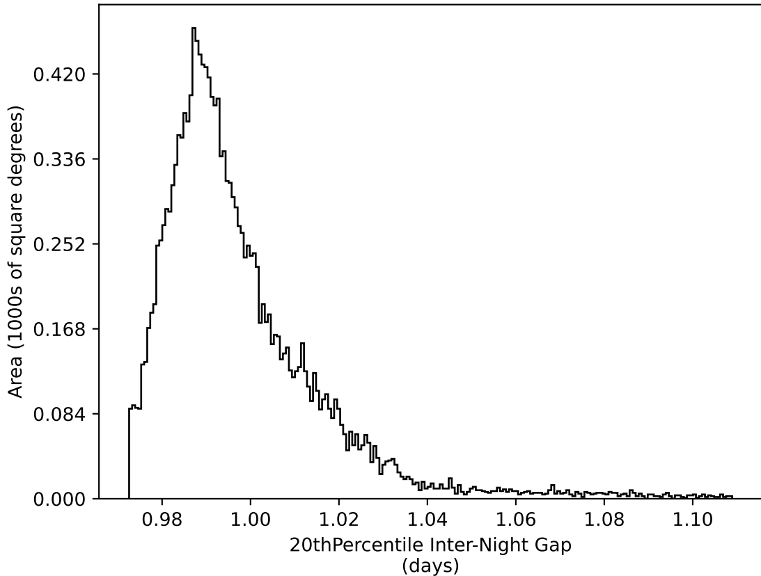
too_elab_r128_d2_griz_v3.4_10yrs WFD all bands: 20thPercentile Inter-Night Gap
