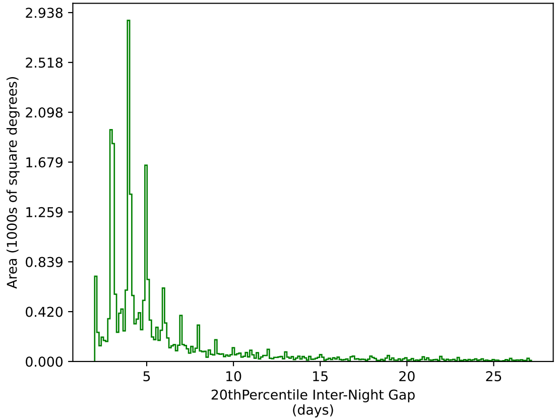
too_elab_r128_d2_griz_v3.4_10yrs All sky g band: 20thPercentile Inter-Night Gap
