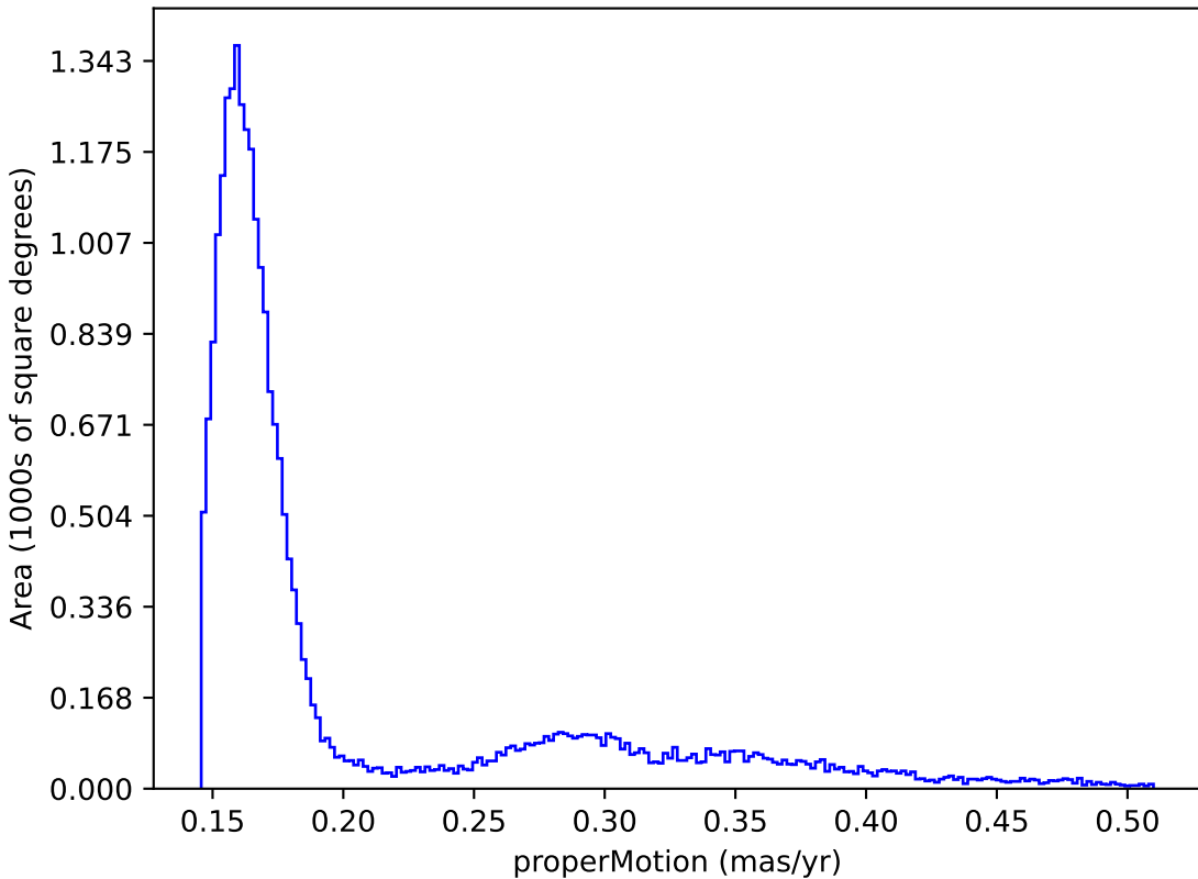
too_elab_r128_d2_griz_v3.4_10yrs : properMotion
