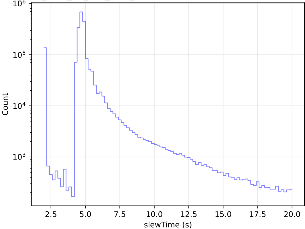
too_elab_r128_d2_griz_v3.4_10yrs All visits: Zoom Slew Time Histogram
