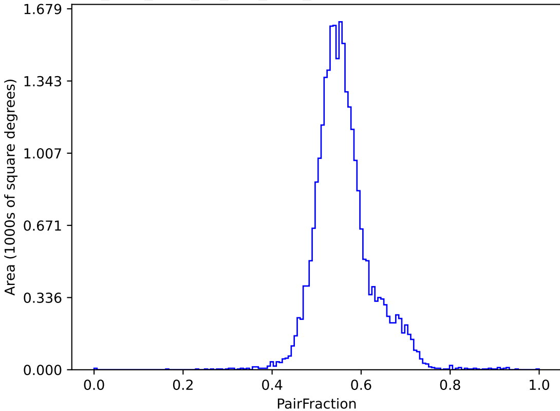
too_elab_r128_d2_griz_v3.4_10yrs (g or r or i): PairFraction
