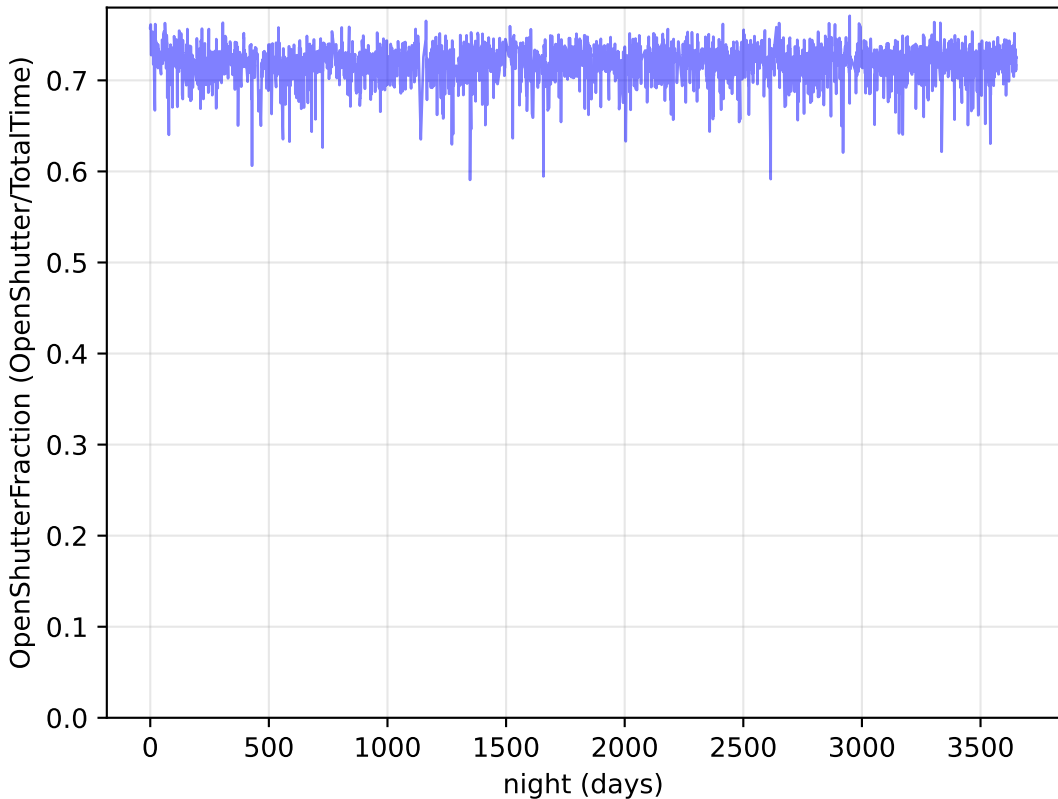
too_elab_r128_d2_griz_v3.4_10yrs : OpenShutterFraction
