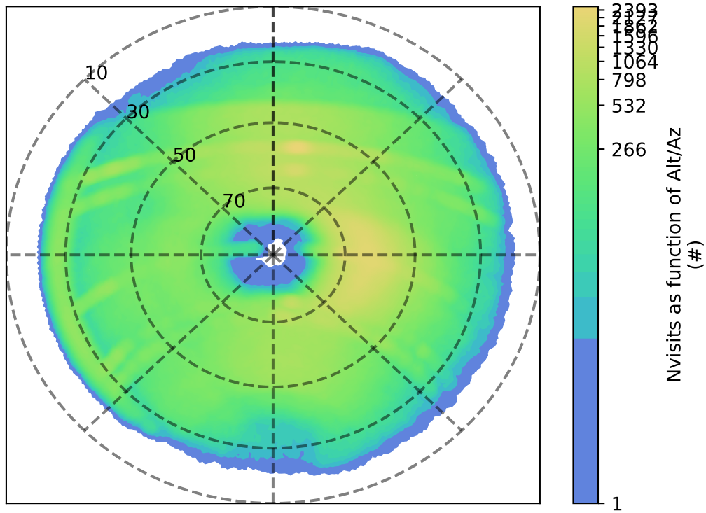
too_elab_r128_d2_griz_v3.4_10yrs r: Nvisits as function of Alt/Az
