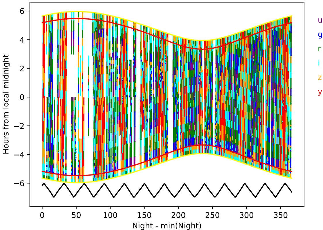
too_elab_r128_d2_griz_v3.4_10yrs year 9-10: Hourglass
