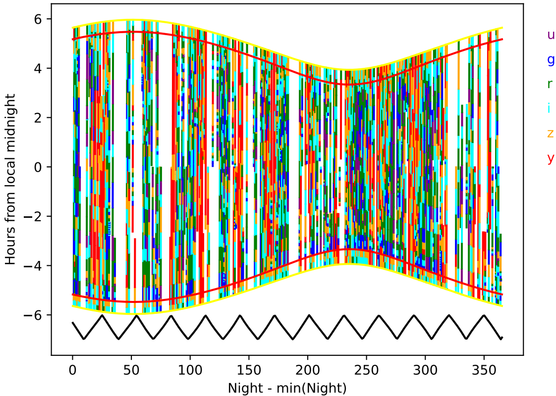
too_elab_r128_d2_griz_v3.4_10yrs year 7-8: Hourglass
