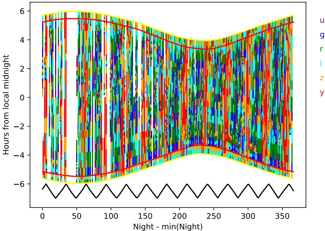
too_elab_r128_d2_griz_v3.4_10yrs year 6-7: Hourglass
