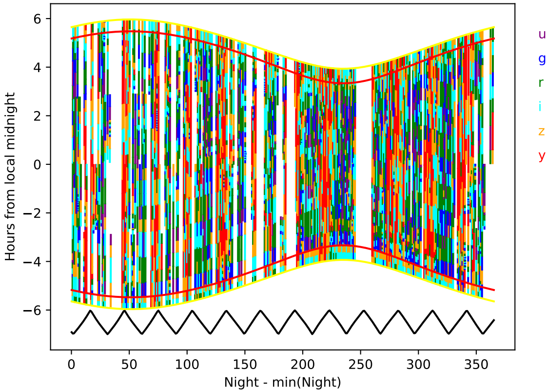
too_elab_r128_d2_griz_v3.4_10yrs year 5-6: Hourglass
