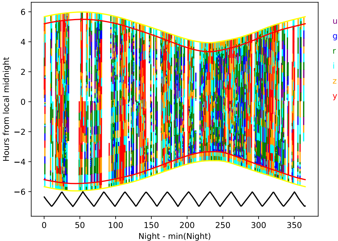
too_elab_r128_d2_griz_v3.4_10yrs year 4-5: Hourglass
