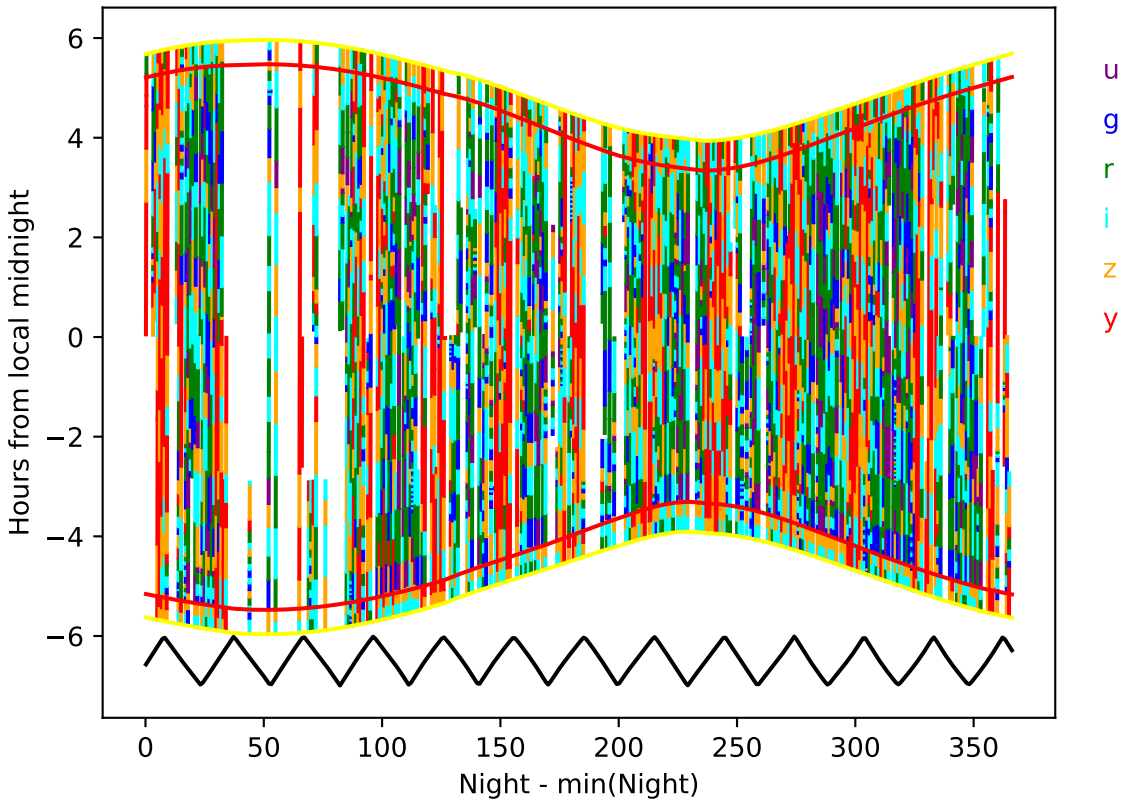
too_elab_r128_d2_griz_v3.4_10yrs year 3-4: Hourglass
