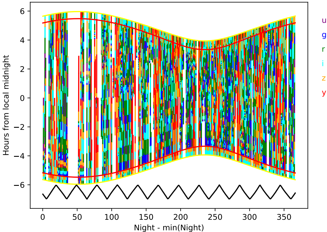
too_elab_r128_d2_griz_v3.4_10yrs year 2-3: Hourglass
