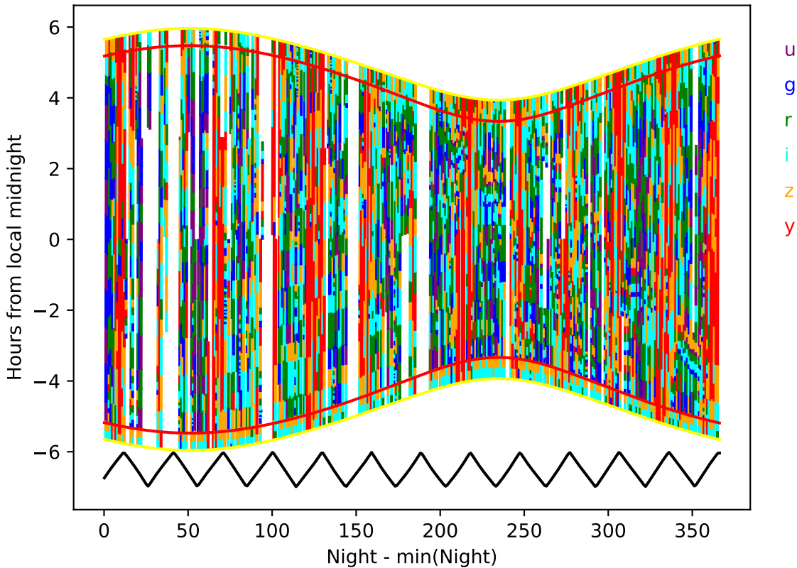
too_elab_r128_d2_griz_v3.4_10yrs year 0-1: Hourglass
