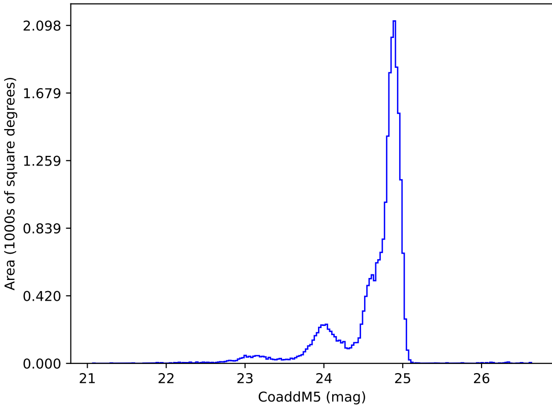
too_elab_r128_d2_griz_v3.4_10yrs y: CoaddM5
