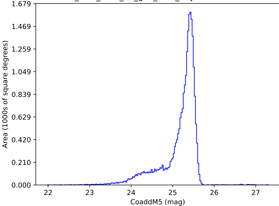
too_elab_r128_d2_griz_v3.4_10yrs u: CoaddM5
